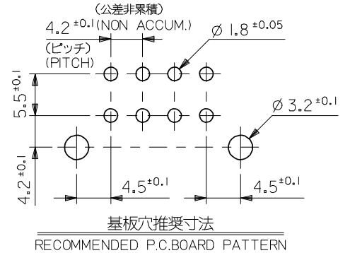
基板取付推奨寸法 RECOMMENDED INSTALLATION PATTERN
