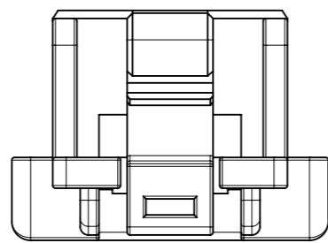
10極形状(1ロック) FIGURE OF 10 CIRCUITS (1 LOCK)
