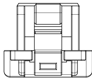
8極形状(1ロック) FIGURE OF 8 CIRCUITS (1 LOCK)
