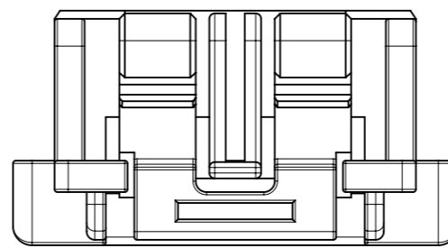
12-18極形状(2ロック) FIGURE OF 12-18 CIRCUITS (2 LOCKS)
