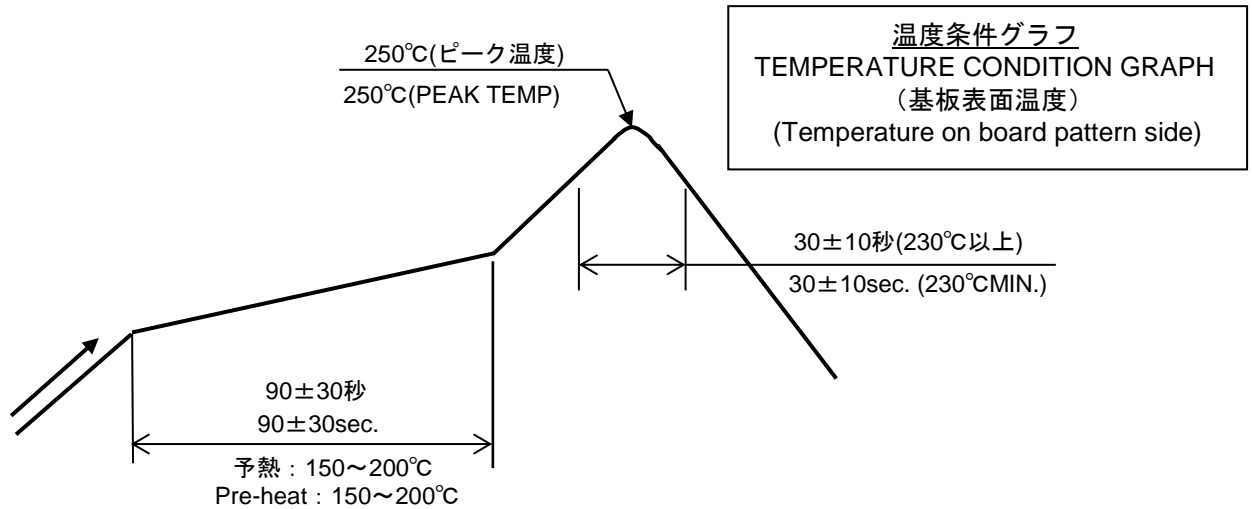
温度条件グラフ TEMPERATURE CONDITION GRAPH (はんだ接合部の基板表面にて測定) (Temperature is measured at the soldering area on the surface of PWB)
