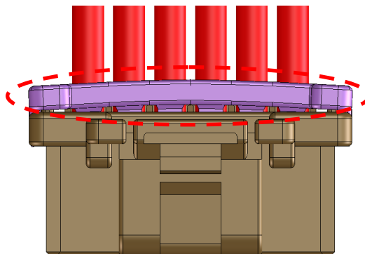
Fig.6-12 the state that the retainer is bending
