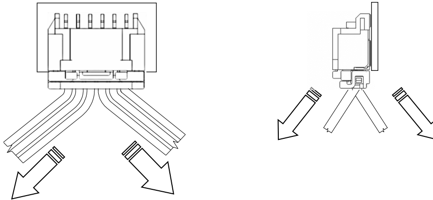
× Fig.9-3-3 Wiring toward more than 2 directions
