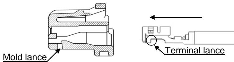
○ Fig.6-2 Right insertion direction
