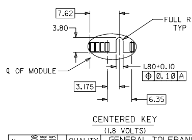
RECOMMENDED MODULE LAYOUT (PER JEDEC STANDARD MO-206, 184 CKT.) UNLESS OTHERWISE SPECIFIED, GENERAL TOLERANCE FOR MODULE = ±0.13
