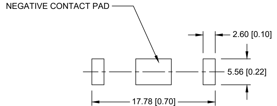
PCB LAYOUT
