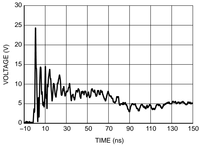
Figure 6. Positive 8 kV ESD Contact Discharge
