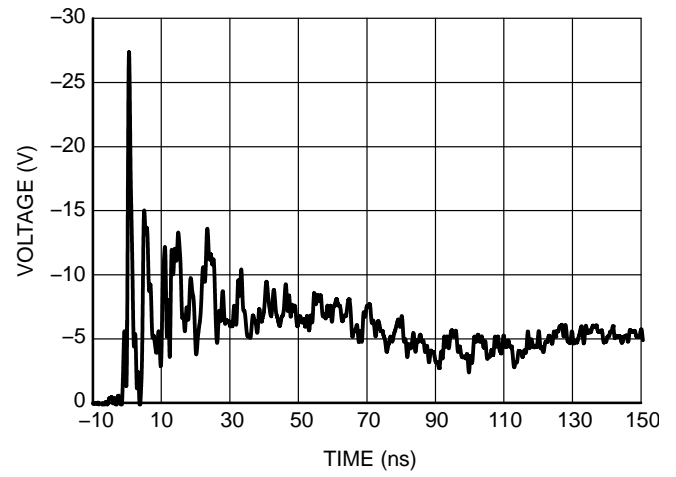
Figure 7. Negative 8 kV ESD Contact Discharge
