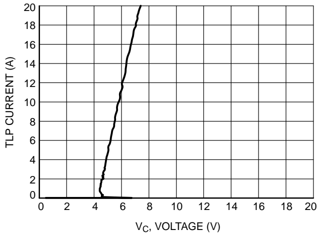
Figure 4. Positive TLP I-V Curve
