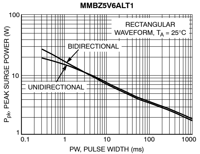
Figure 9. Maximum Non-repetitive Surge Power, P_{pk(NOM)} versus PW
