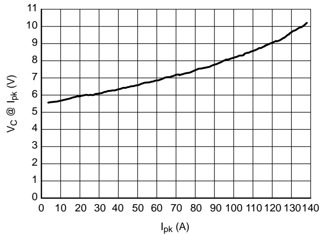
Figure 4. Clamping Voltage vs. Peak Pulse Current ( t_p = 8/20 \mu s ), Pin 2 to Pin 1
