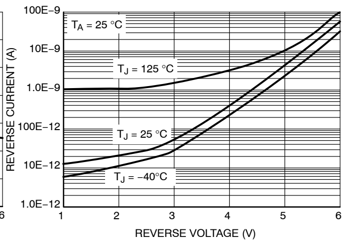
Figure 2. Typical Reverse Current vs. Reverse Voltage
