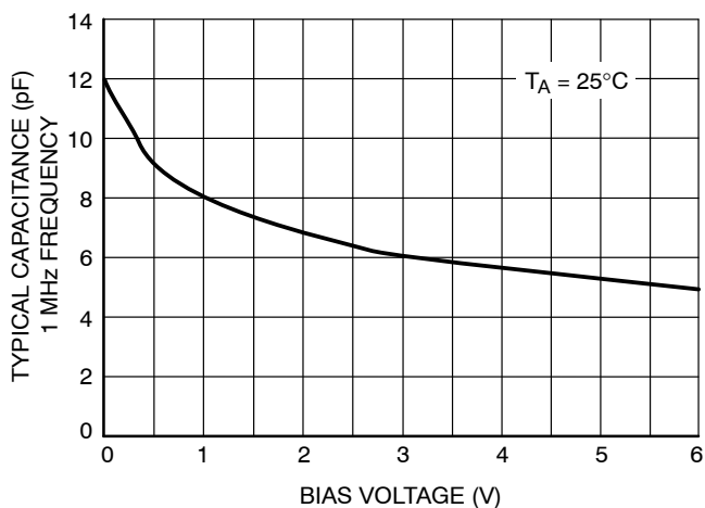
Figure 1. Capacitance
