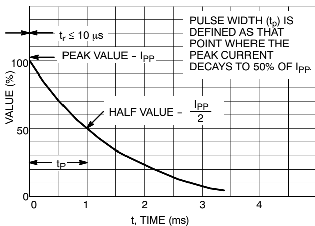
Figure 4. Pulse Waveform
