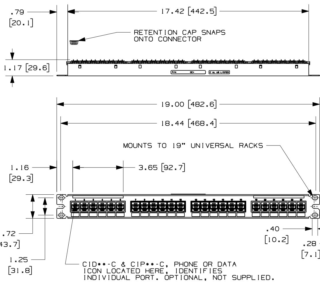
FIGURE 1 DP6 PLUS 24 PORT PATCH PANEL
