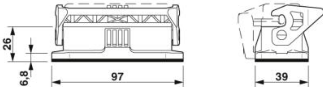
Dimensional drawing
