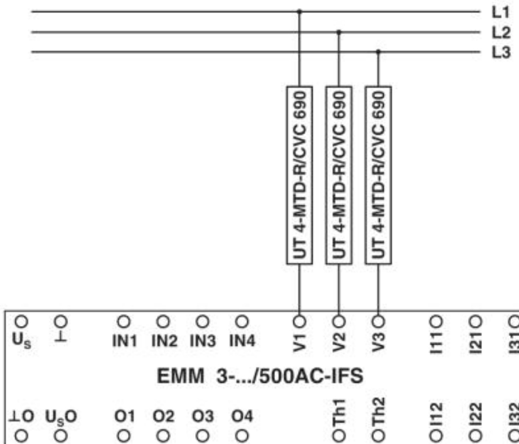
Connection diagram
