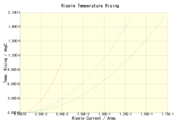
C1608X7R2A222K080AA(100kHz) C1608X7R2A222K080AA(500kHz) C1608X7R2A222K080AA(1MHz)
