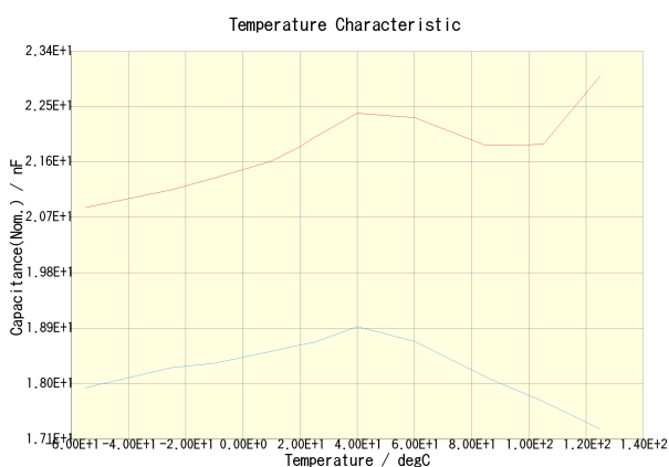
C2012X7R2A223K125AA(DC Bias = 0V) C2012X7R2A223K125AA(DC Bias = 50V)
