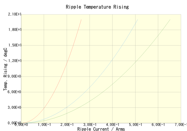
C2012X7R2A223K125AA(100kHz) C2012X7R2A223K125AA(500kHz) C2012X7R2A223K125AA(1MHz)
