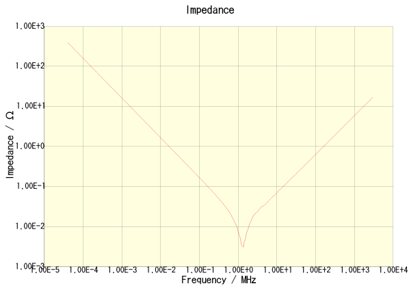
C3216X5R1A106M160AB
