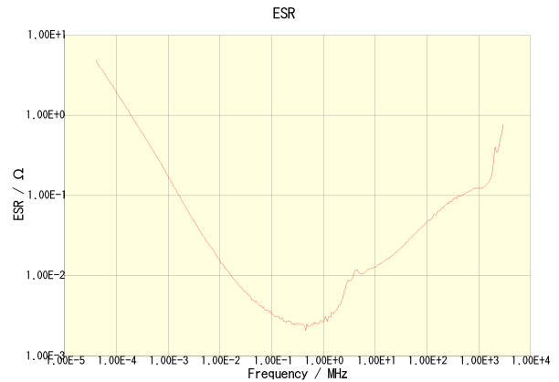
C3216X5R1A106M160AB
