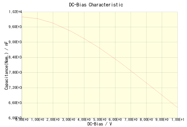
C3216X5R1A106M160AB
