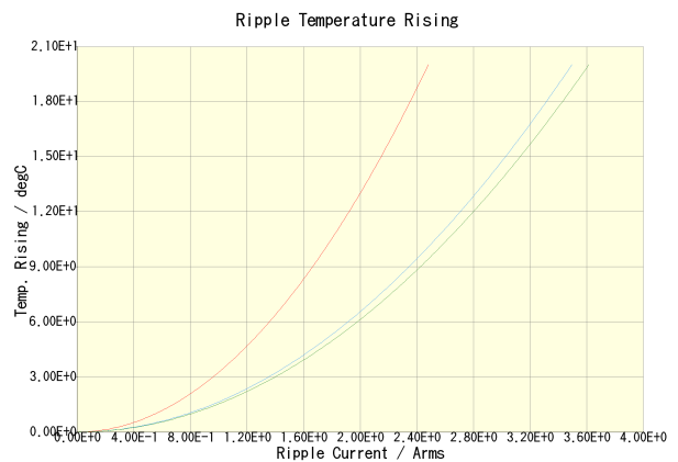
C3216X7R1E225K160AA(100kHz) C3216X7R1E225K160AA(500kHz) C3216X7R1E225K160AA(1MHz)
