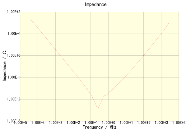
CKG57NX5R1C107M500JH
