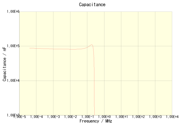
CKG57NX5R1C107M500JH
