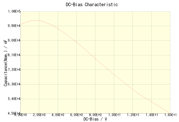
CKG57NX5R1C107M500JH
