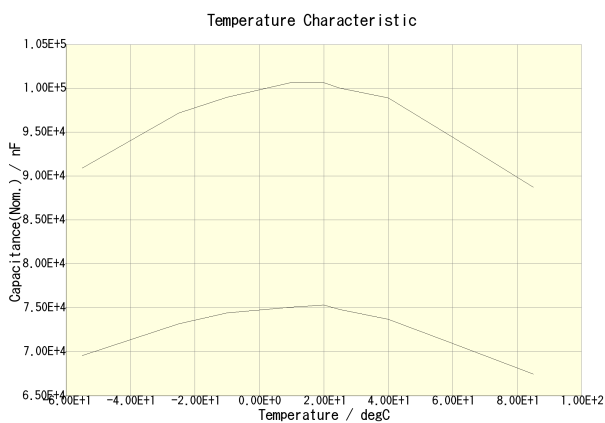
CKG57NX5R1C107M500JH(DC Bias = 8V) CKG57NX5R1C107M500JH(DC Bias = 8V)
