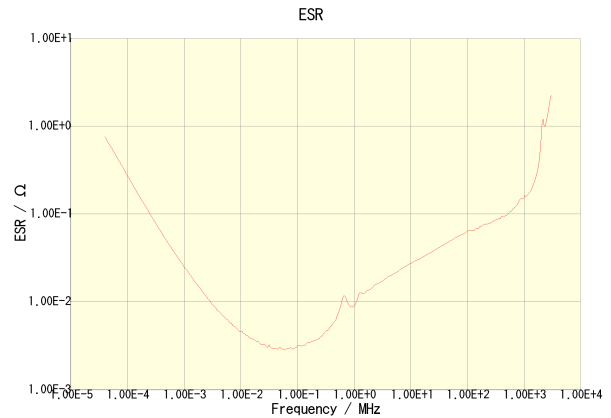
CKG57NX5R1C107M500JH
