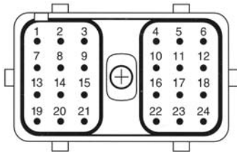
In-line Receptacle
