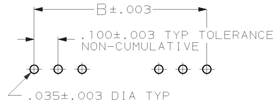
RECOMMENDED HOLE LAYOUT
