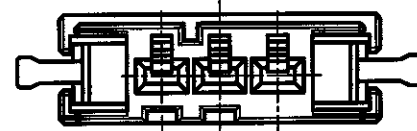
5-178288-3 (P/N 1-178288-3 ONLY) (KEYING: X)
