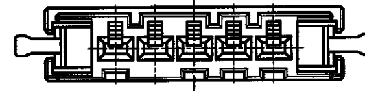
(P/N 2-178288-6,-8) (KEYING: Y)
