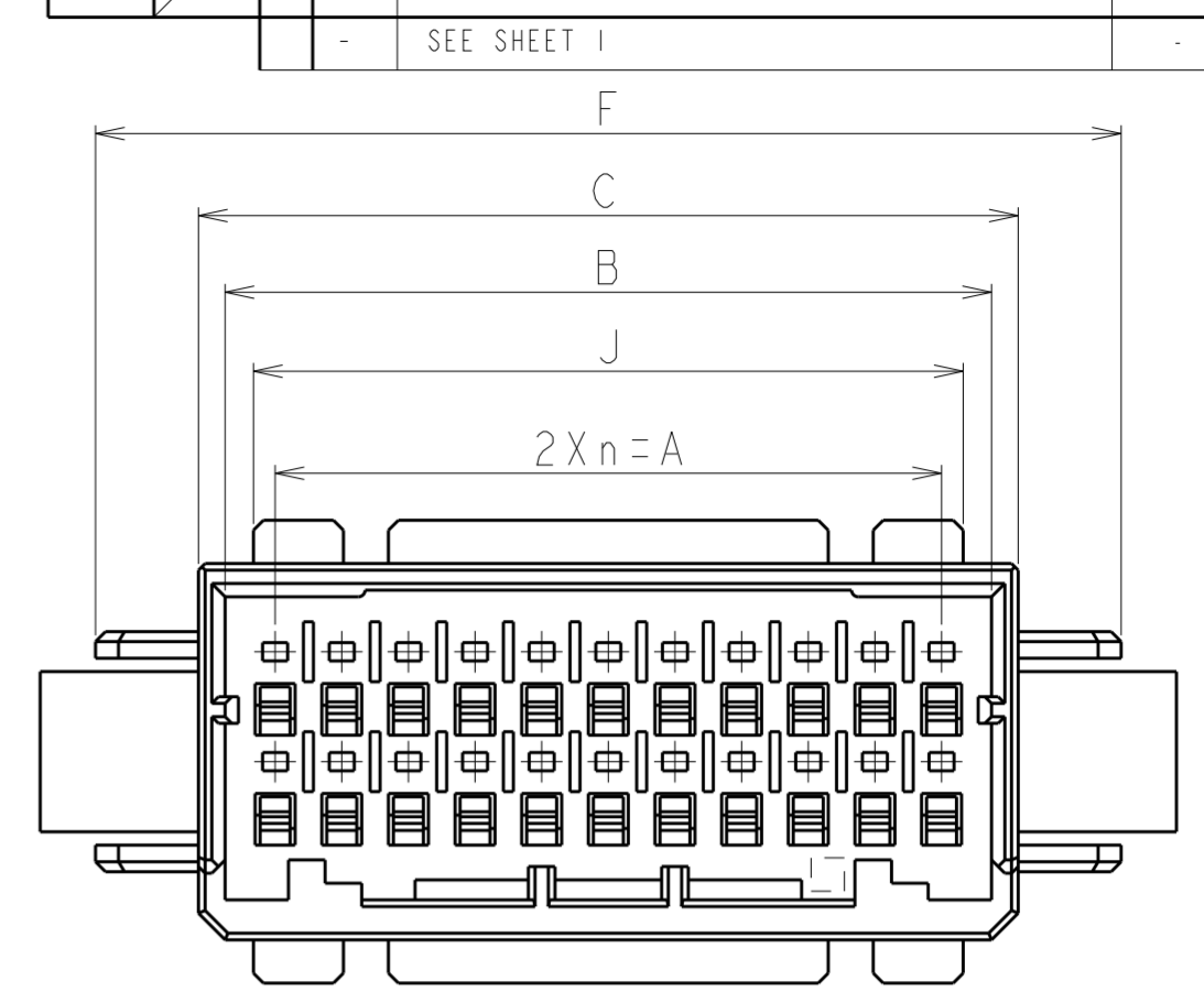
22POS(X-KEY): 1-1903128-1
