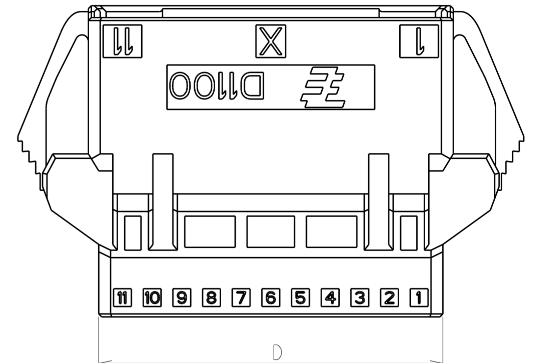
22POS(X-KEY): 1-1903128-1
