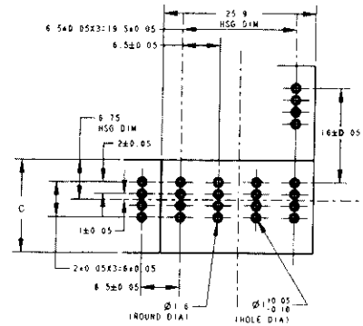
PC Board Layout Board thickness: 1.6±0.2
