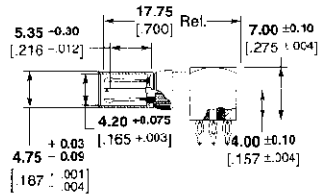
Part No. 148386-1
