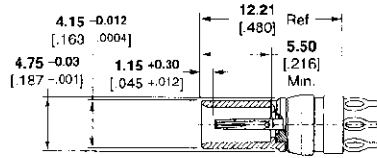
Part No. 148385-1
