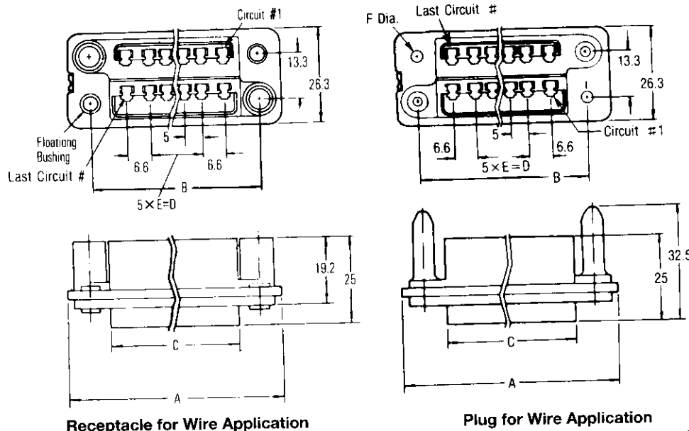
Receptacle for Wire Application
