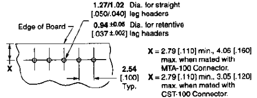
Recommended Mounting Hole Size for 1.57 [.062] PC Board
