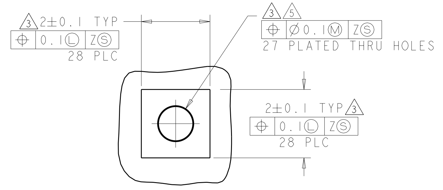
DETAIL D SCALE 15:1
