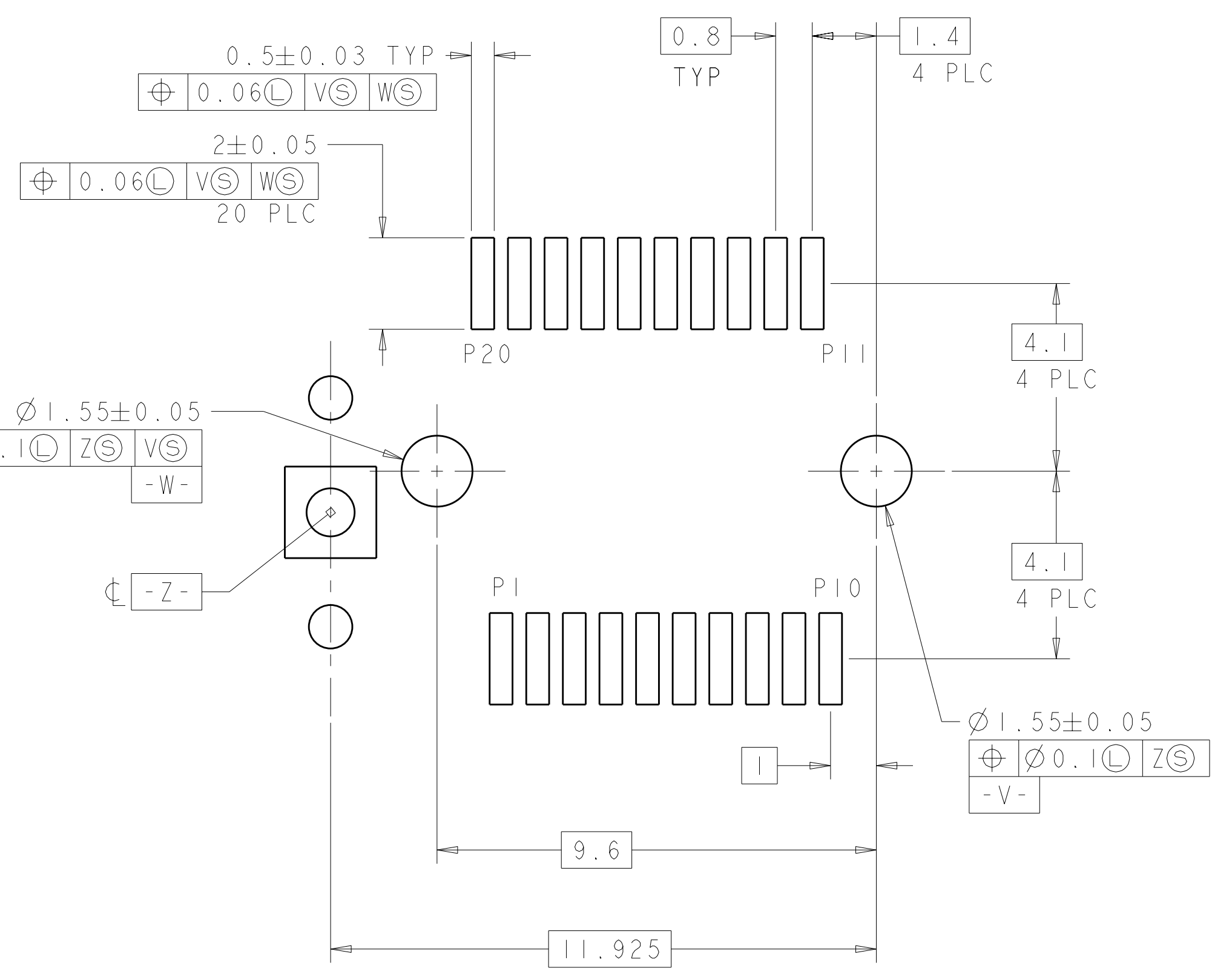
PT CONNECTOR RECOMMENDED PCB CONFIGURATION SCALE 10:1
