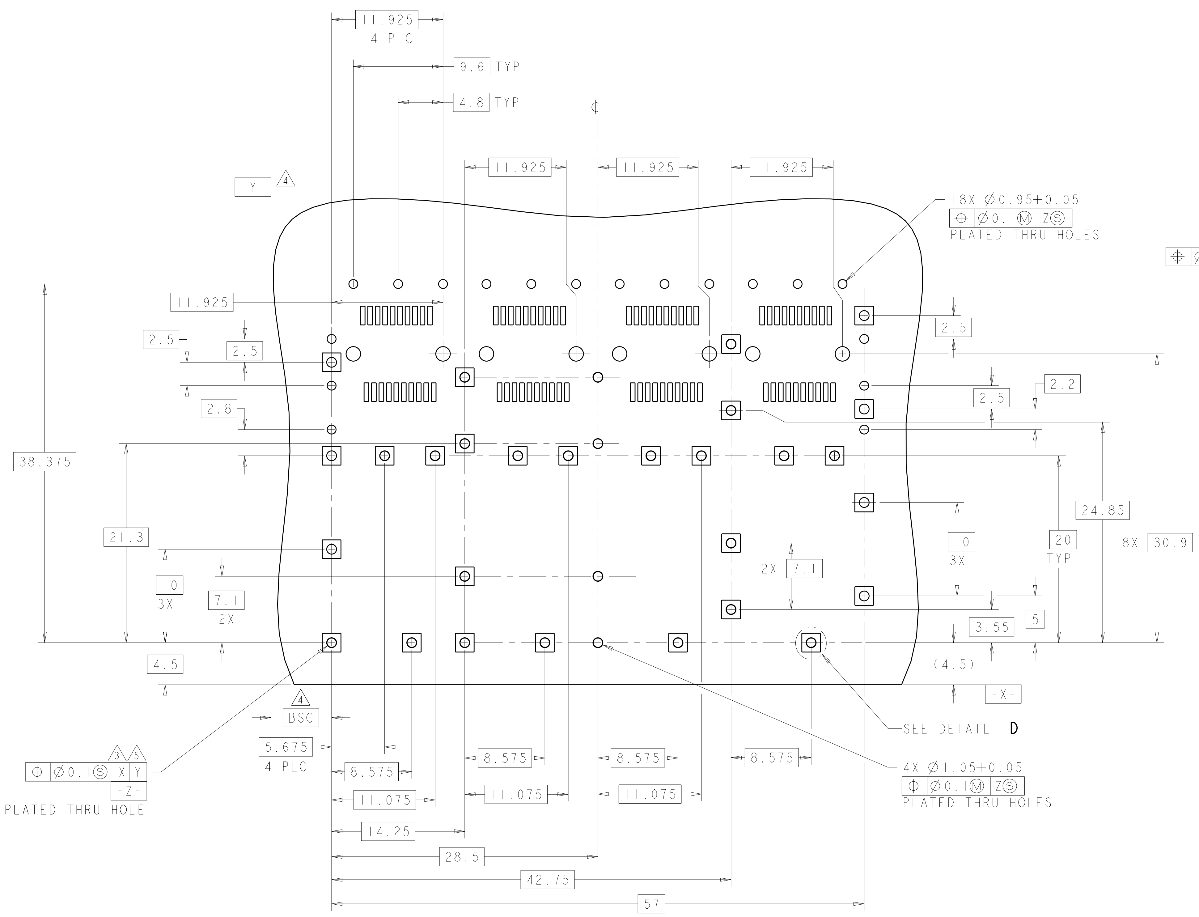
1658744-1 RECOMMENDED PCB CONFIGURATION SCALE 4:1
