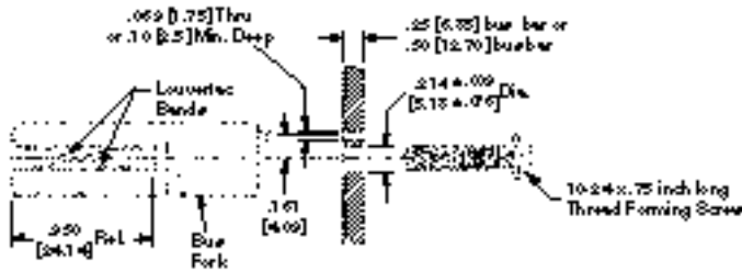
Part Number 194257-1
