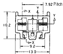
Section Y-Y
