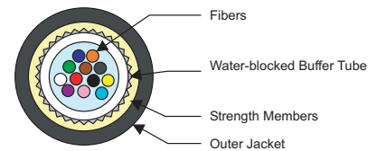
12-Fiber Cable Cross Section
