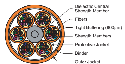
72-Fiber Cable Cross Section
