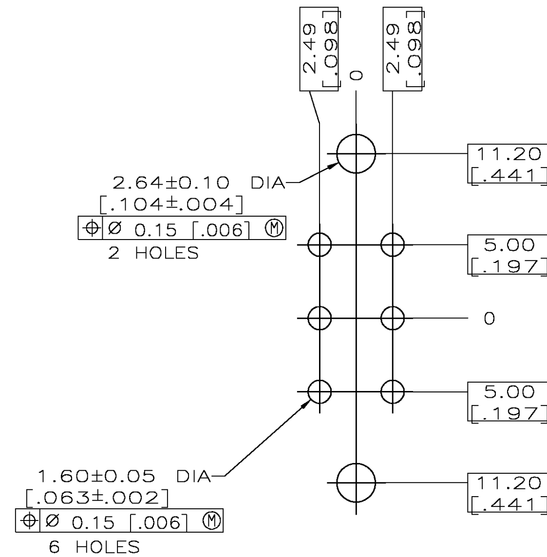
RECOMMENDED LAYOUT
