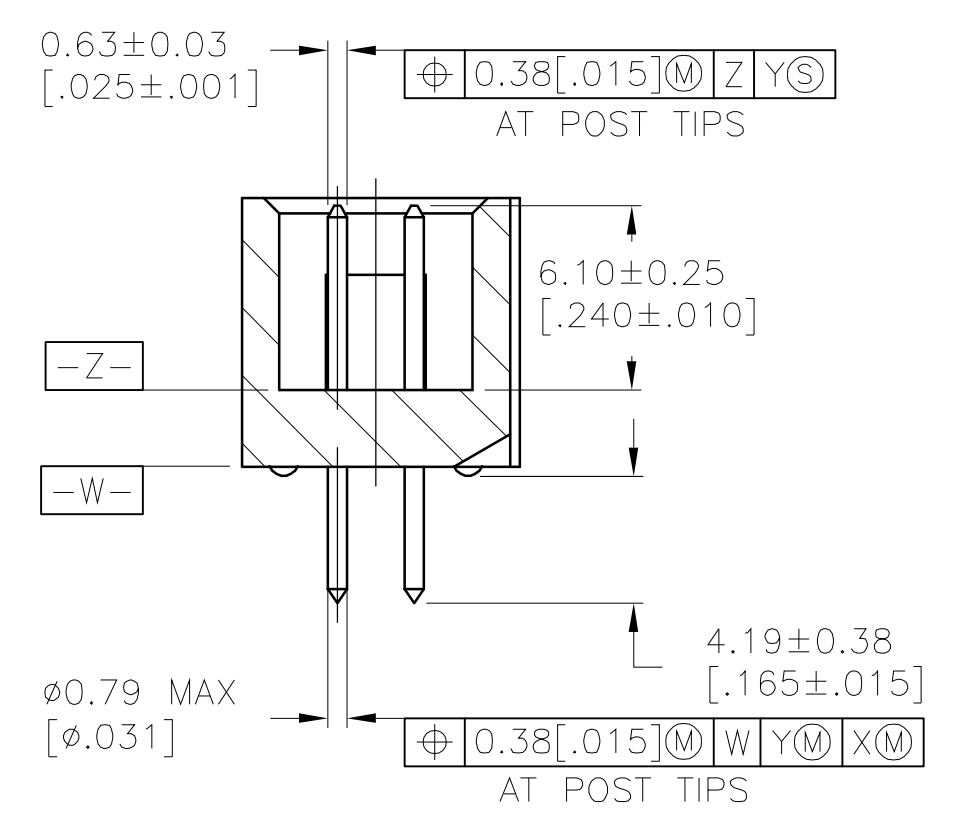
SECTION U-U
