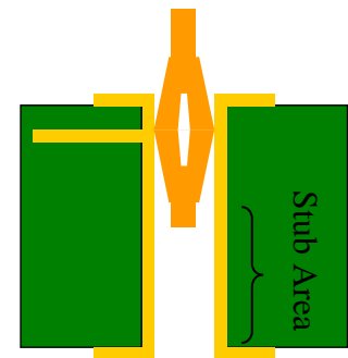
Figure 7: Via Stub
