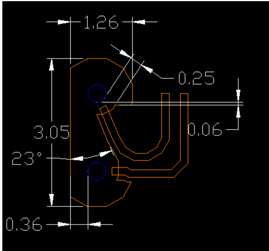
Figure 6: Daughtercard Breakout Antipad, Right-Side
