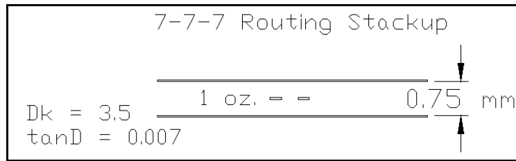
Figure 15: 7-7-7 Routing
