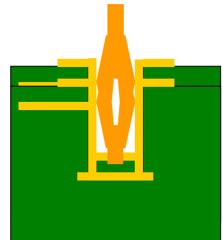
Figure 9: Blind Via
