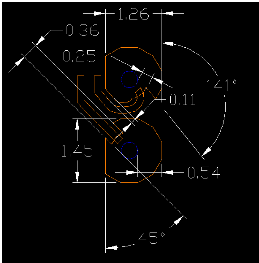
Figure 5: Daughtercard Breakout Antipad, Left-Side
