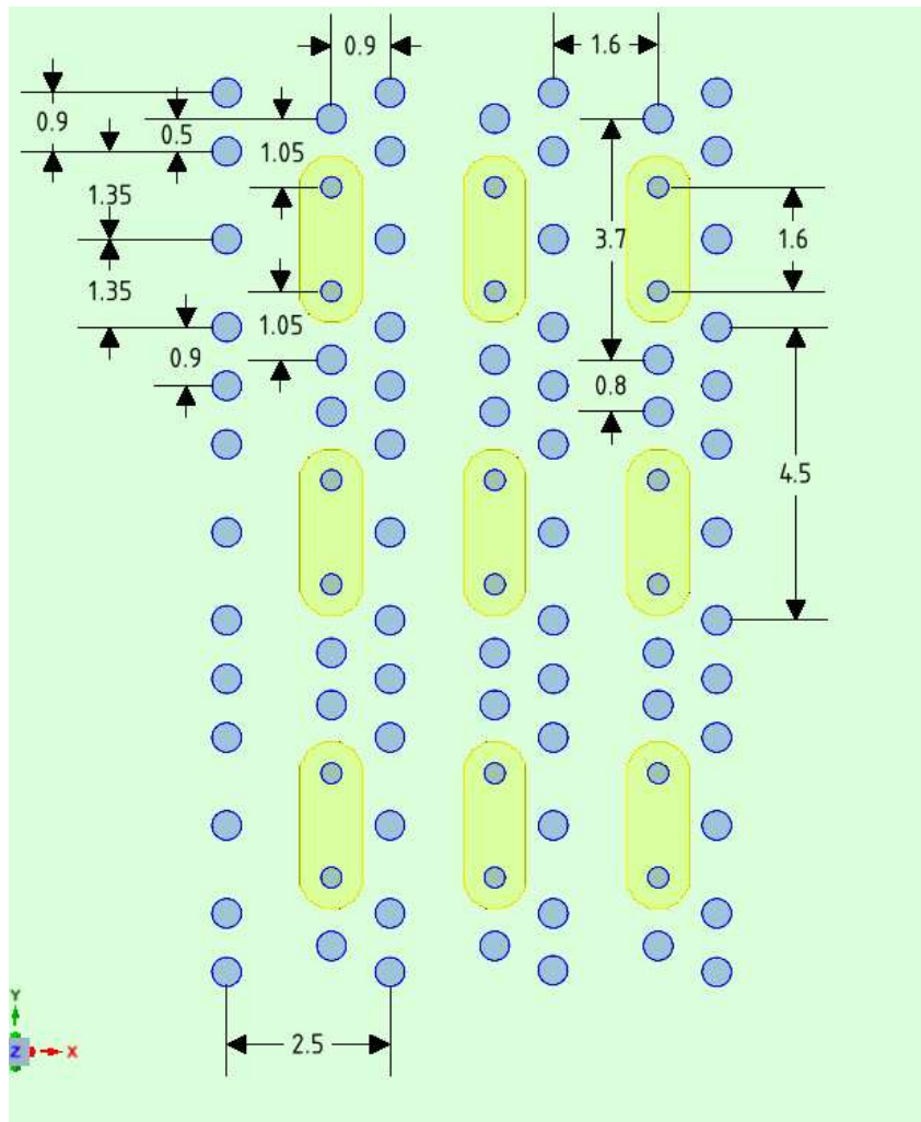
Figure 2: STRADA Whisper Daughtercard Footprint Dimensions
