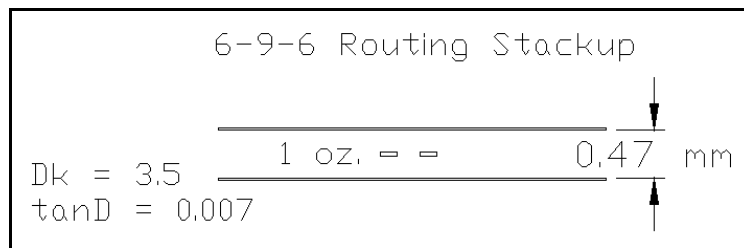
Figure 16: 6-9-6 Routing
