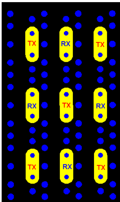
Figure 14: Interstitial Pinout
