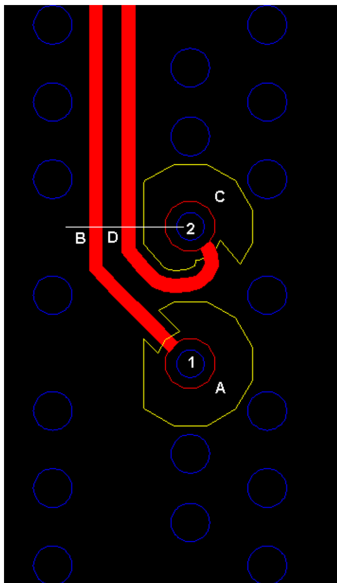
Figure 12: Example Breakout
