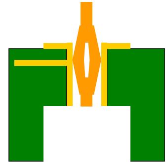
Figure 8: Counterbored Via
