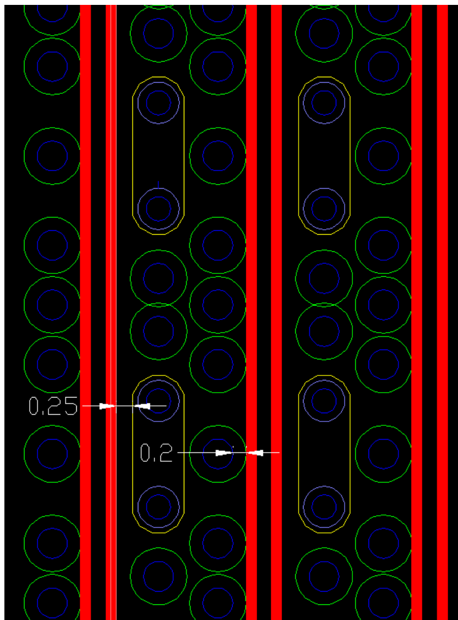
Figure 10: Daughtercard Channel Routing with 6-9-6 trace
