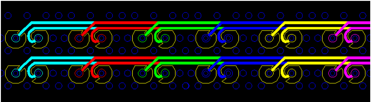
Figure 13: Typical Layer Count Breakdown for 6-pair Daughtercard Connector
