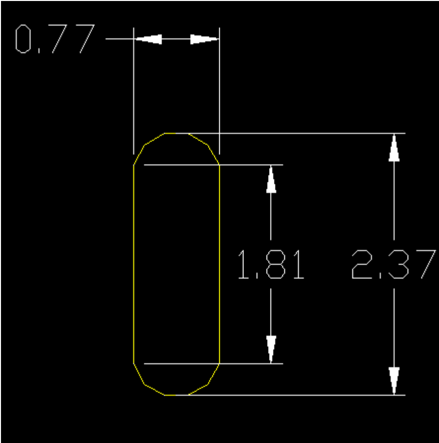
Figure 4: Daughtercard Antipad Geometry
