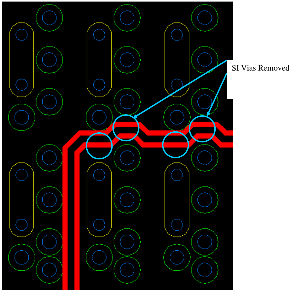
Figure 11: Horizontal Daughtercard Channel Routing
