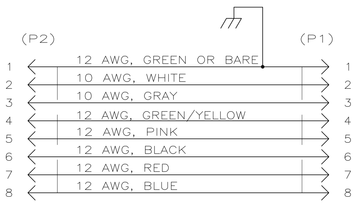
WIRING DIAGRAM 8 WIRE
