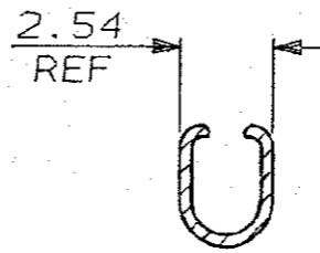
SECTION X-X
