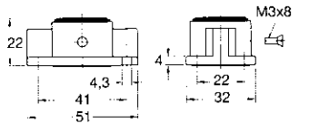
Montageausschnitt/Panel cut-out 21 x 21
