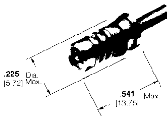
RG-405 Semi-Rigid/.086 Cable Part No. 413249-1
