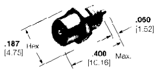
Part No. 413020-1
