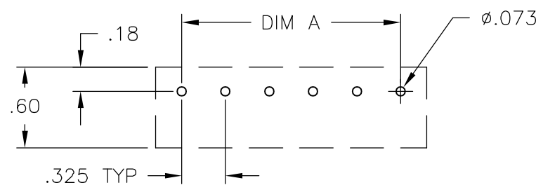
RECOMMENDED HOLE LAYOUT TOLERANCE ±.002, UNLESS OTHERWISE SPECIFIED
