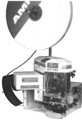
AMP-O-LECTRIC Model G, No. 354500 Series with Tyco Electronics Crimp Quality Monitor
