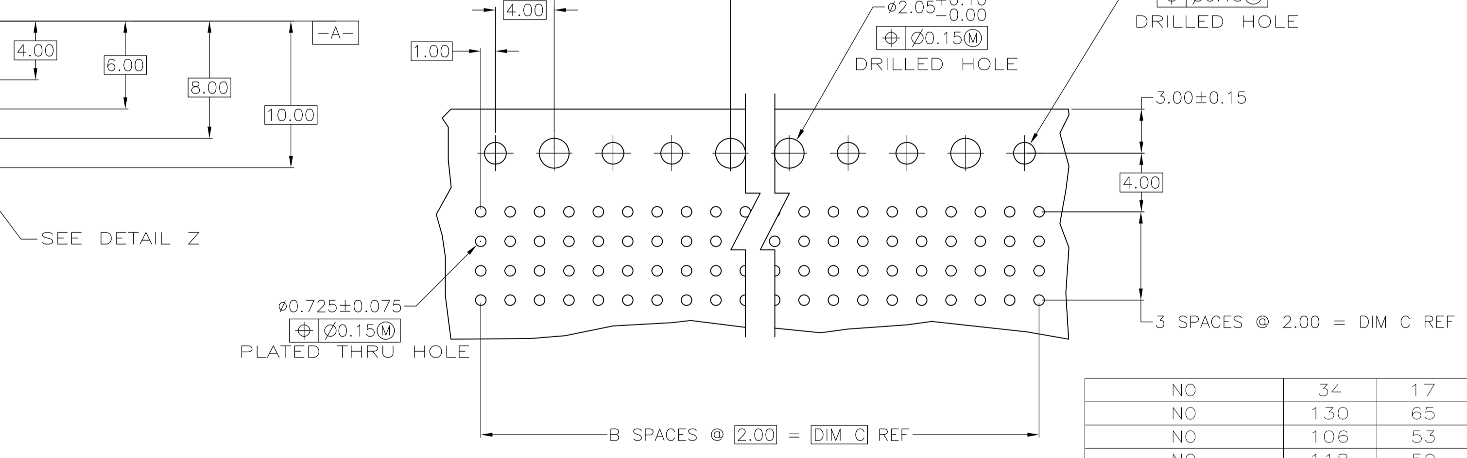
RECOMMENDED CIRCUIT PATTERN PER IPC-D300 TYPE II, CLASS C (COMPONENT SIDE)
