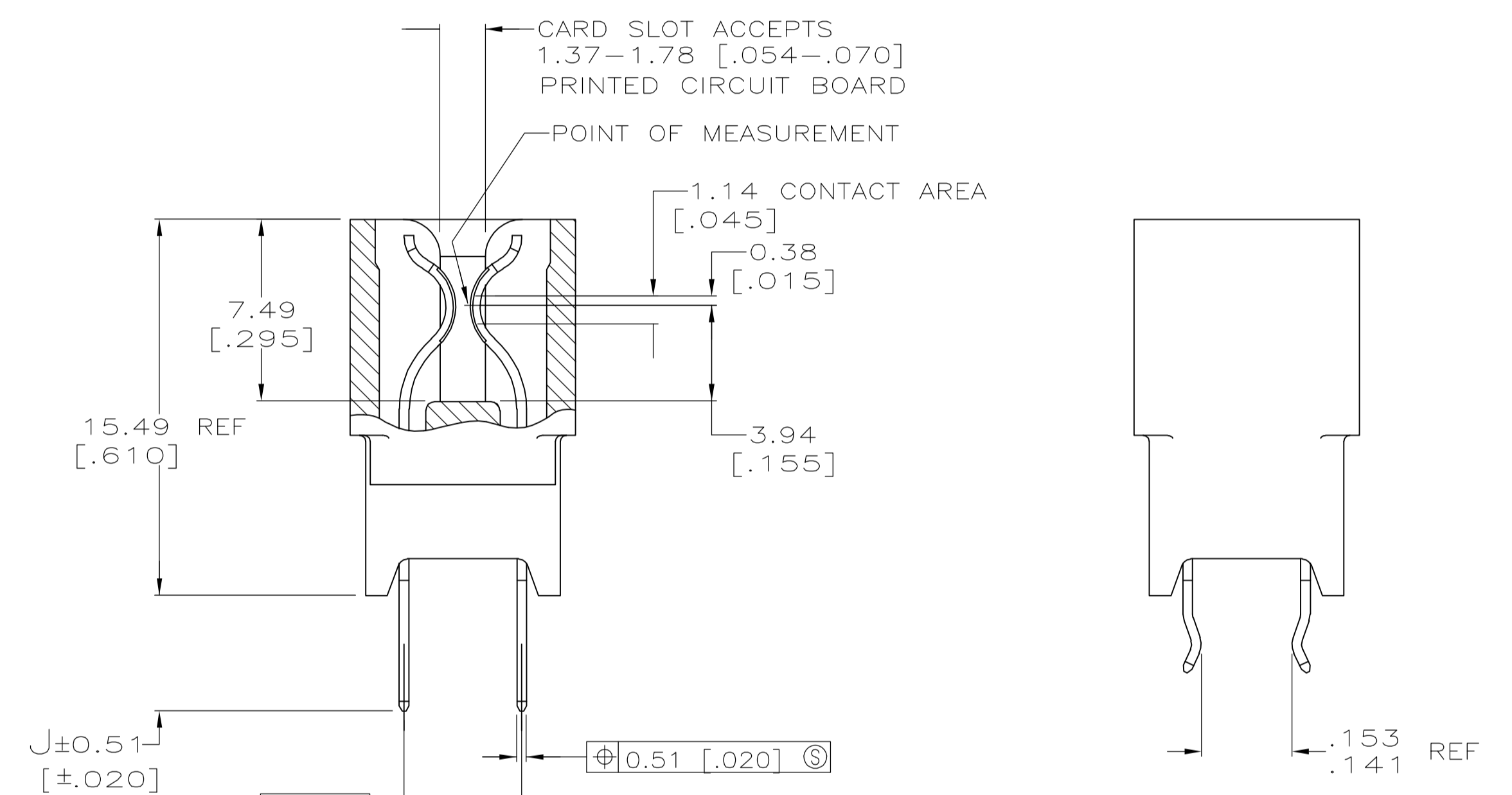
BOARD RETENTION FEATURE 8-5530843-3 ONLY
