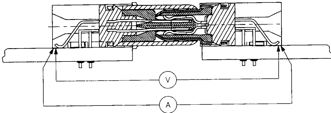
Figure 4 Termination Resistance Measurement Points
