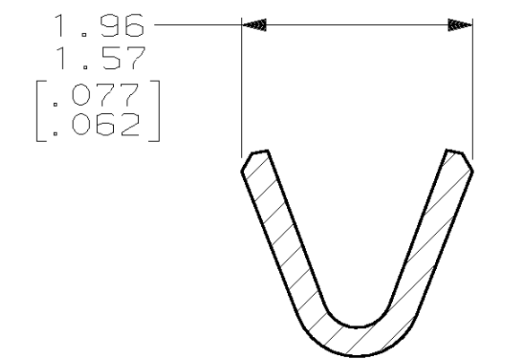
SECTION Y-Y WIRE BARREL SCALE 20:1
