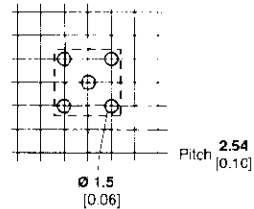
Recommended Mounting Holes
