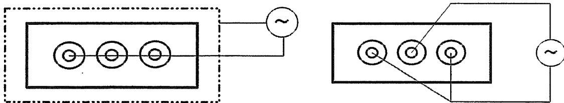
Fig.4 Measurement of Insulation resistance and Withstand voltage
