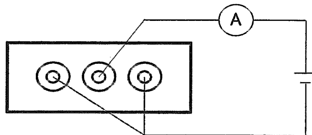
Fig.5 Measuring leak current between the adjacent contacts
