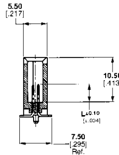
Section C - C (Rotated 90°)
