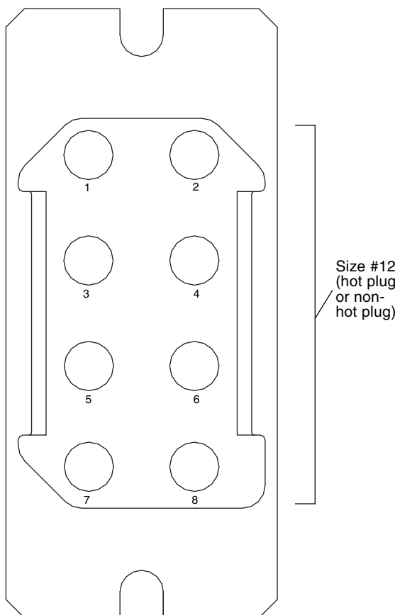
Pin housing (rear face) Pin contact insertion side. Pin connector rear face cavity identification
