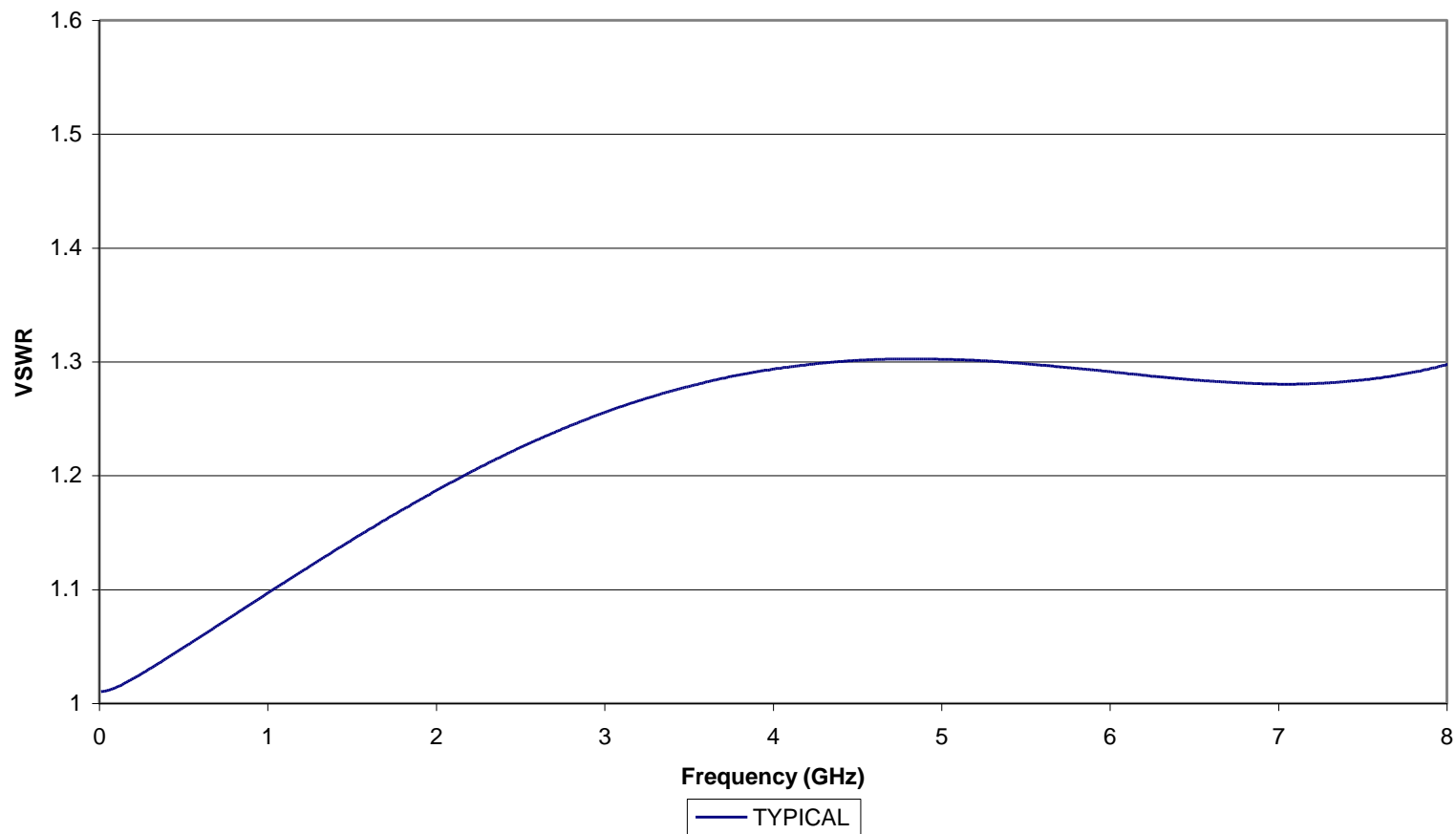
Typical VSWR of KOAXXA SMA-PS-1B (2081202-5) RD-316 cable
