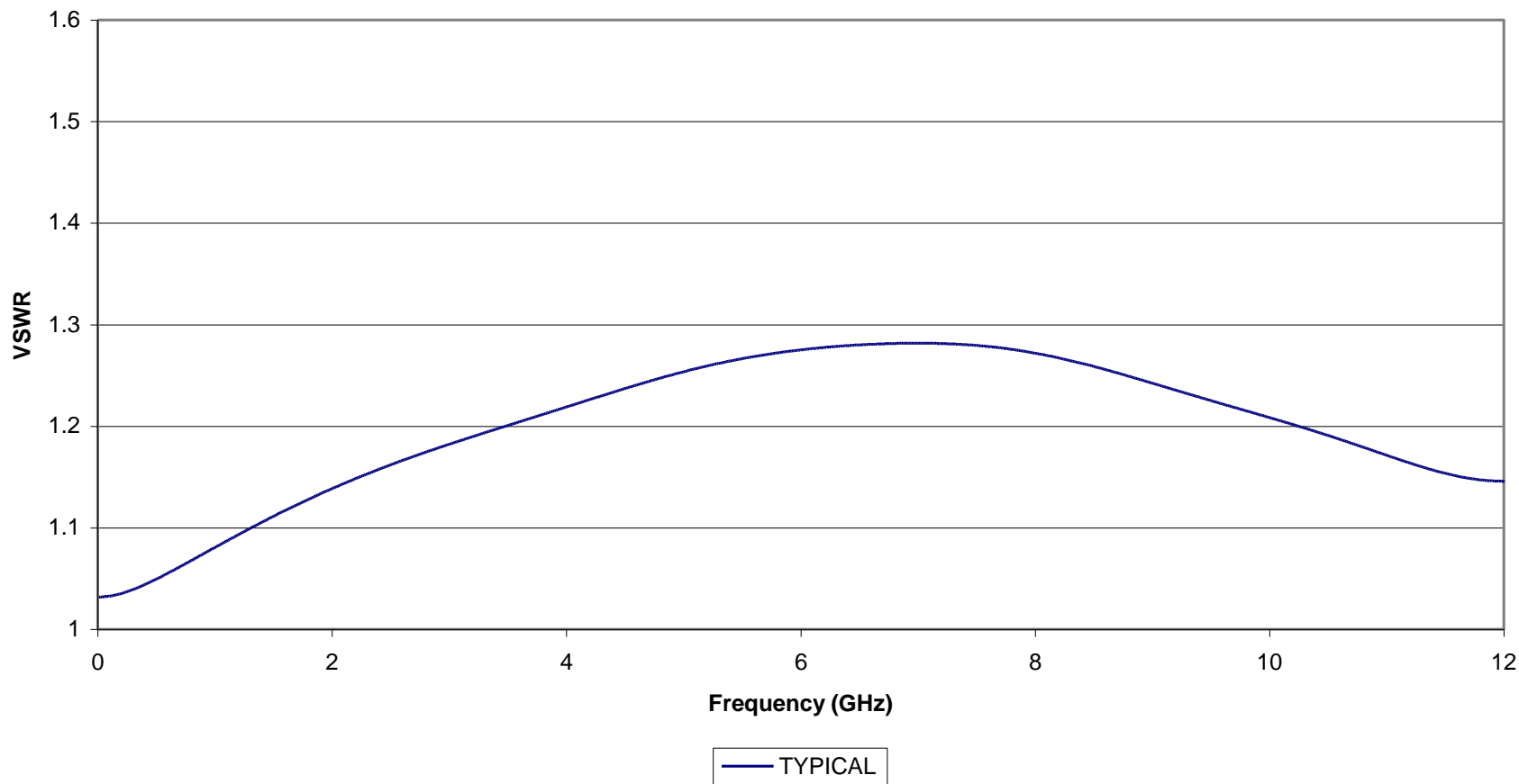
TYPICAL VSWR of KOAXXA SMA-JS-1G (2081205-7) RG-58 Cable
