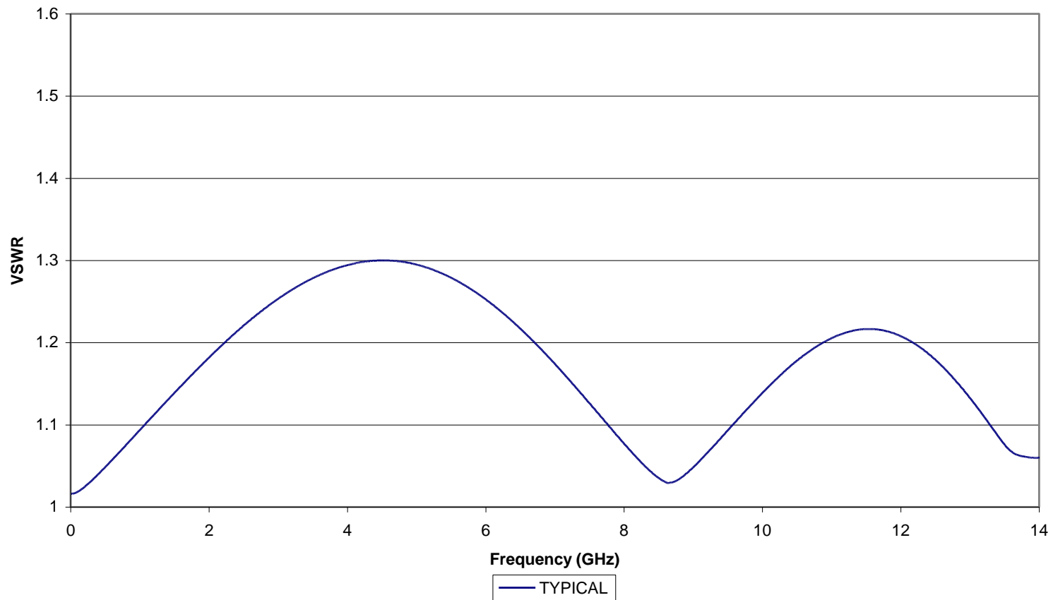
Typical VSWR of KOAXXA SMA-PR-1F (2081203-3) RG-316 Cable
