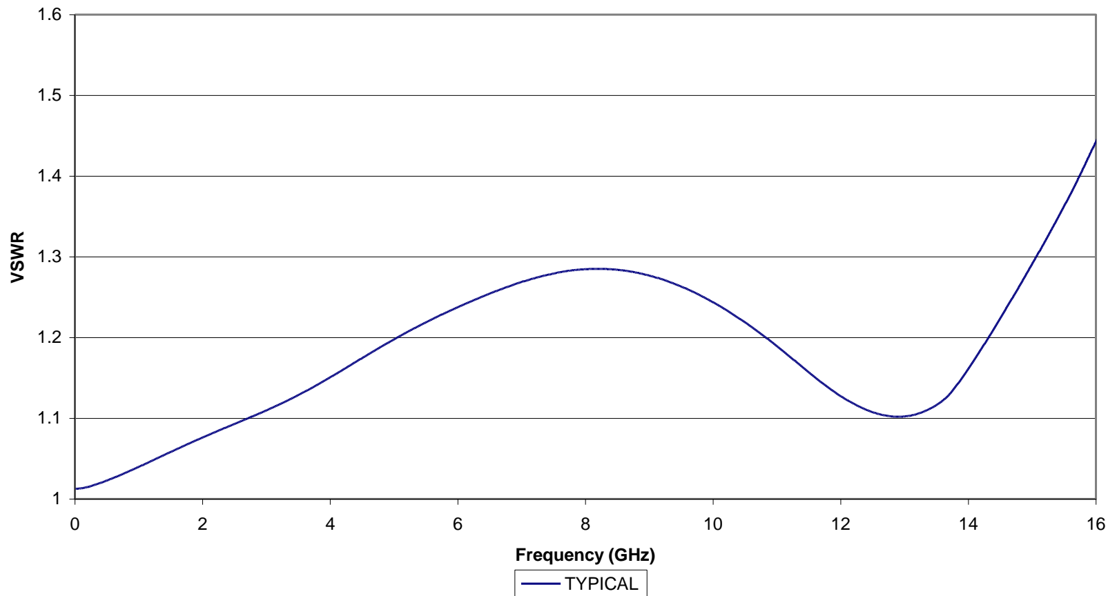
TYPICAL VSWR OF KOAXXA SMA-PR-1C (2081203-9) RG-405 Cable
