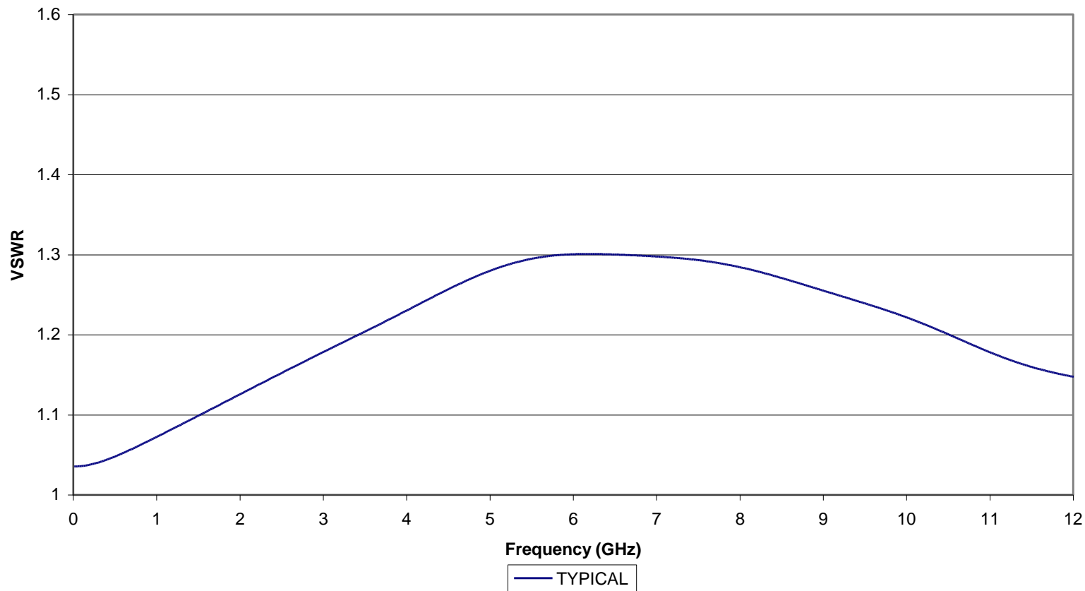
TYPICAL VSWR OF KOAXXA SMA-PS-1G (2081202-7) RG-58 Cable
