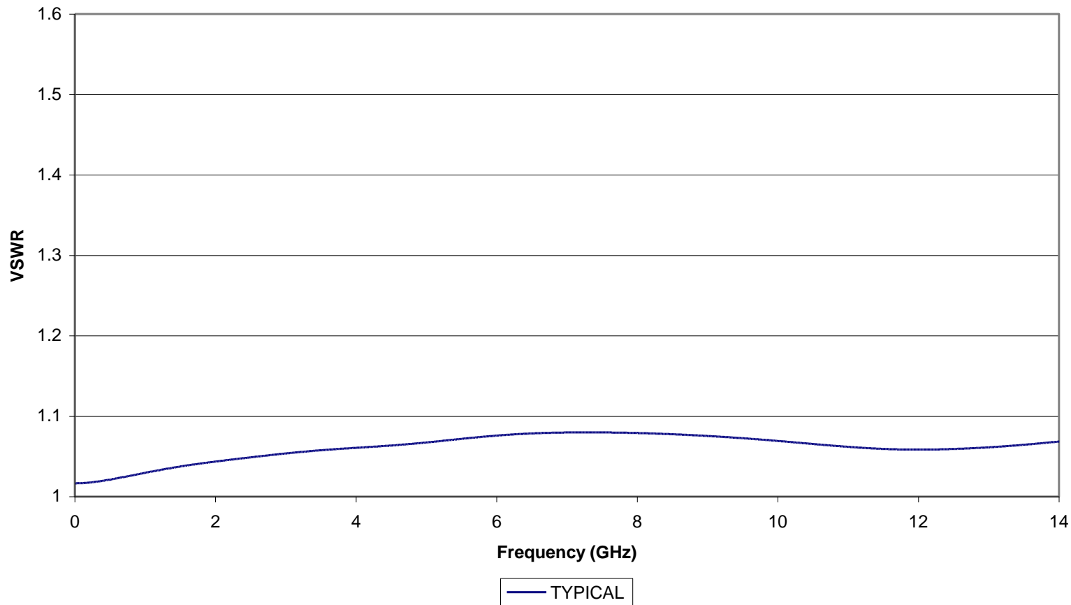
TYPICAL VSWR OF KOAXXA SMA-JB-1C (2081204-9) RG-405 Cable
