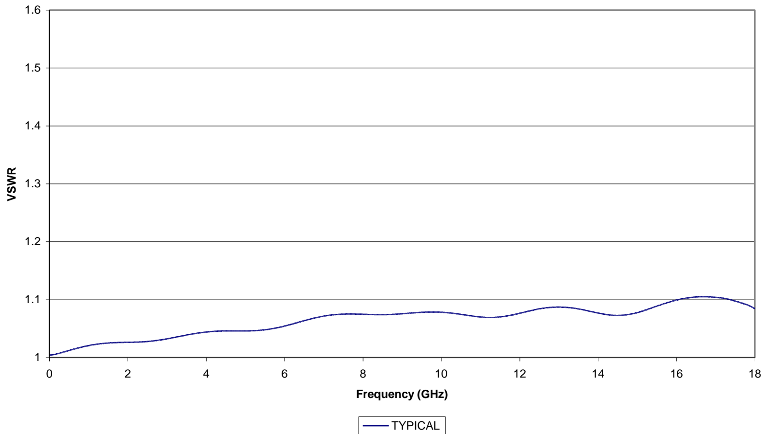
Typical VSWR of KOAXXA SMA-JB-1A (2081204-1) RG-402 Cable
