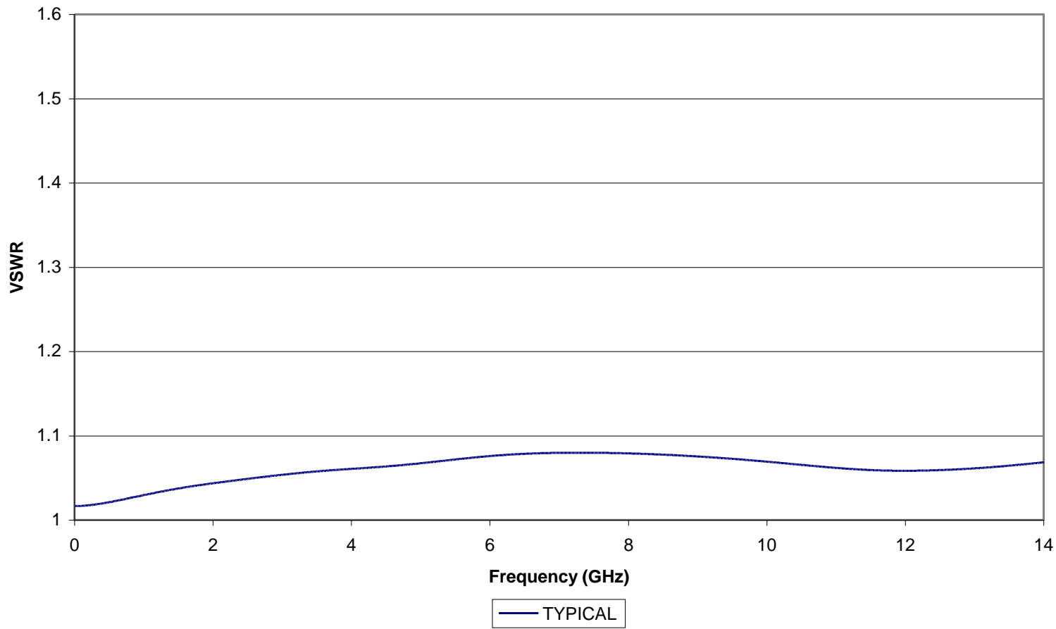
TYPICAL VSWR OF KOAXXA SMA-JS-1C (2081205-9) RG-405 Cable
