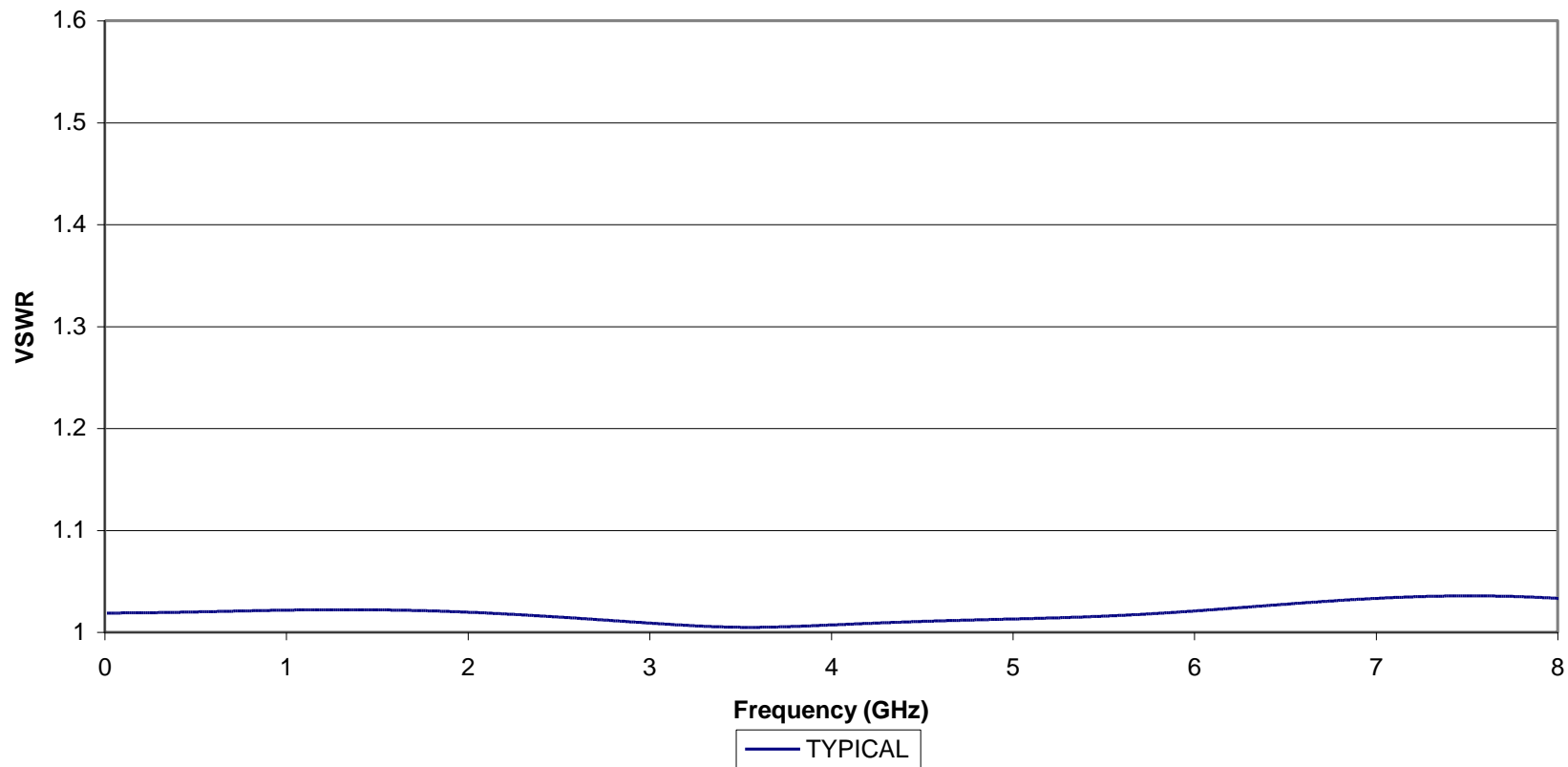
TYPICAL VSWR OF KOAXXA SMA-JS-1D (1-2081205-1) RG-178 Cable
