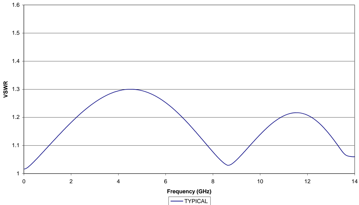
Typical VSWR of KOAXXA SMA-PR-1B (2081203-5) RD-316 Cable
