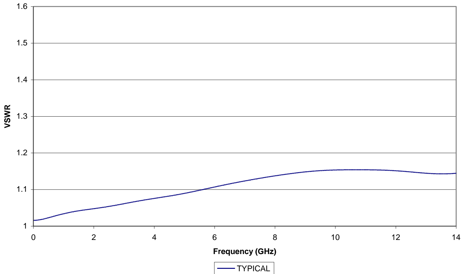
TYPICAL VSWR OF KOAXXA SMA-PS-1C (2081202-9) RG-405 Cable
