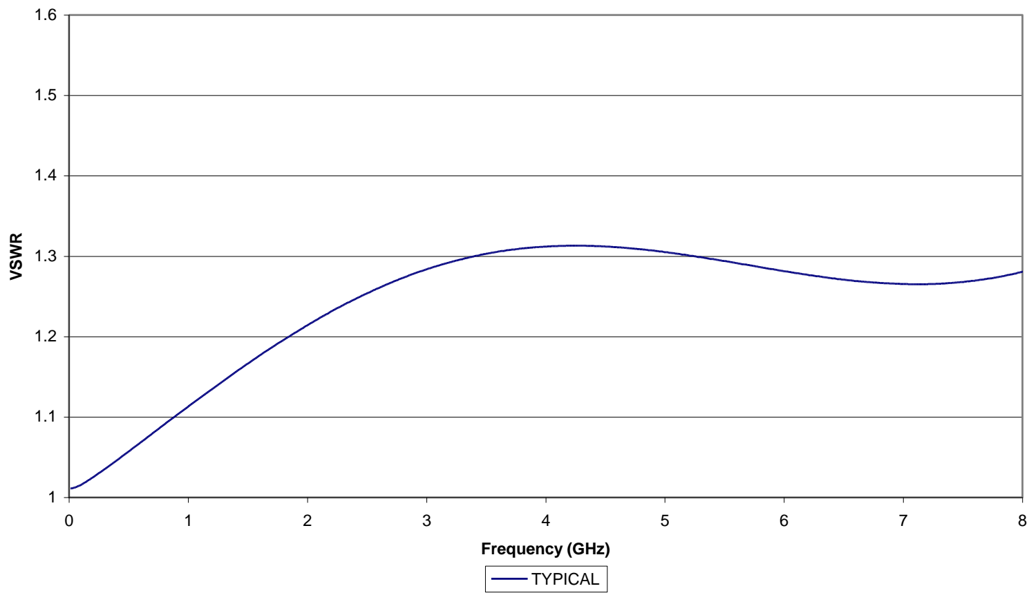
Typical VSWR of KOAXXA SMA-JB-1B (2081204-5) RD-316 cable
