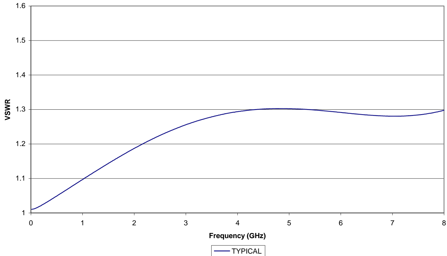
Typical VSWR of KOAXXA SMA-PS-1F (2081202-3) RG-316 cable
