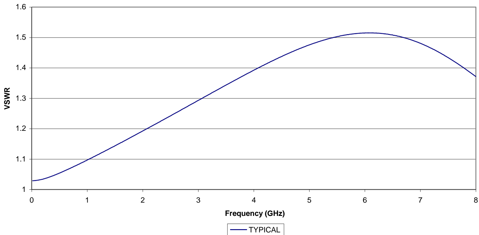
Typical VSWR OF KOAXXA SMA-PR-1D (1-2081203-1) RG-178 Cable
