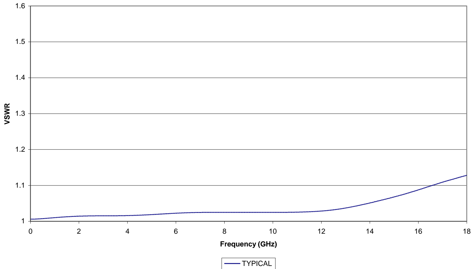
Typical VSWR of KOAXXA SMA-PS-1A (2081202-1) RG-402 Cable
