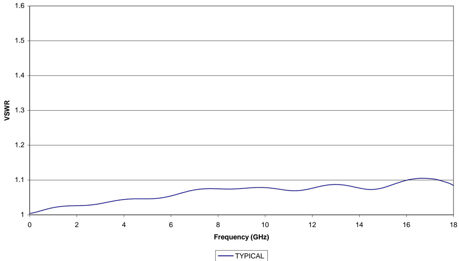
Typical VSWR of KOAXXA SMA-JS-1A (2081205-1) RG-402 Cable
