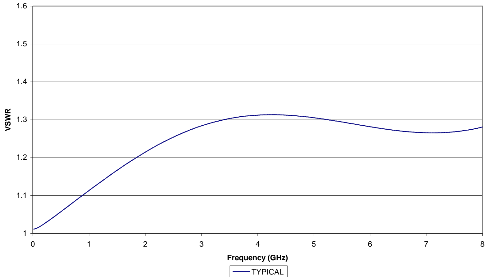
Typical VSWR of KOAXXA SMA-JS-1F (2081205-3) RG-316 cable
