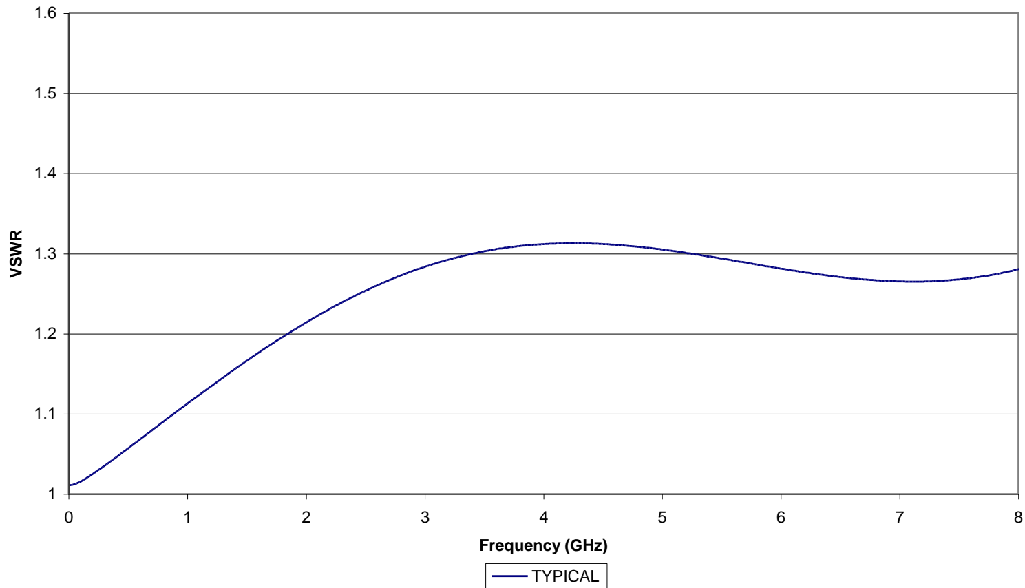
Typical VSWR of KOAXXA SMA-JB-1F (2081204-3) RG-316 cable
