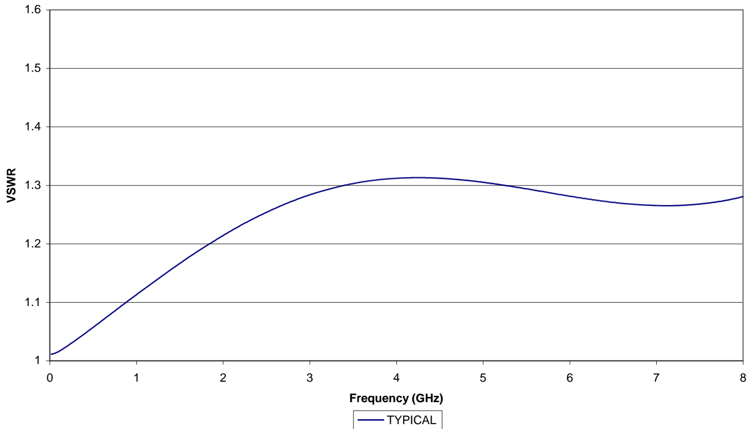
Typical VSWR of KOAXXA SMA-JS-1B (2081205-5) RD-316 cable
