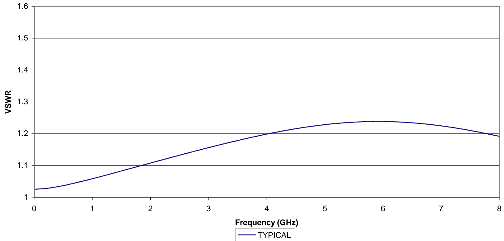
TYPICAL VSWR OF KOAXXA SMA-PS-1D (1-2081202-1) RG-178 Cable
