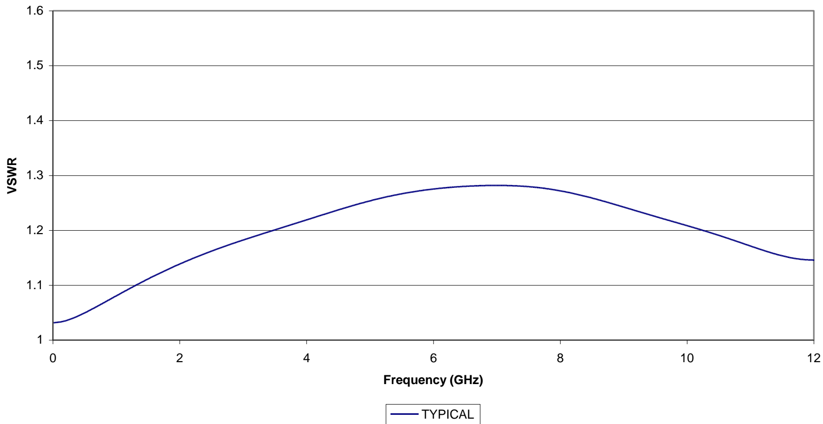
TYPICAL VSWR of KOAXXA SMA-JB-1G (2081204-7) RG-58 Cable
