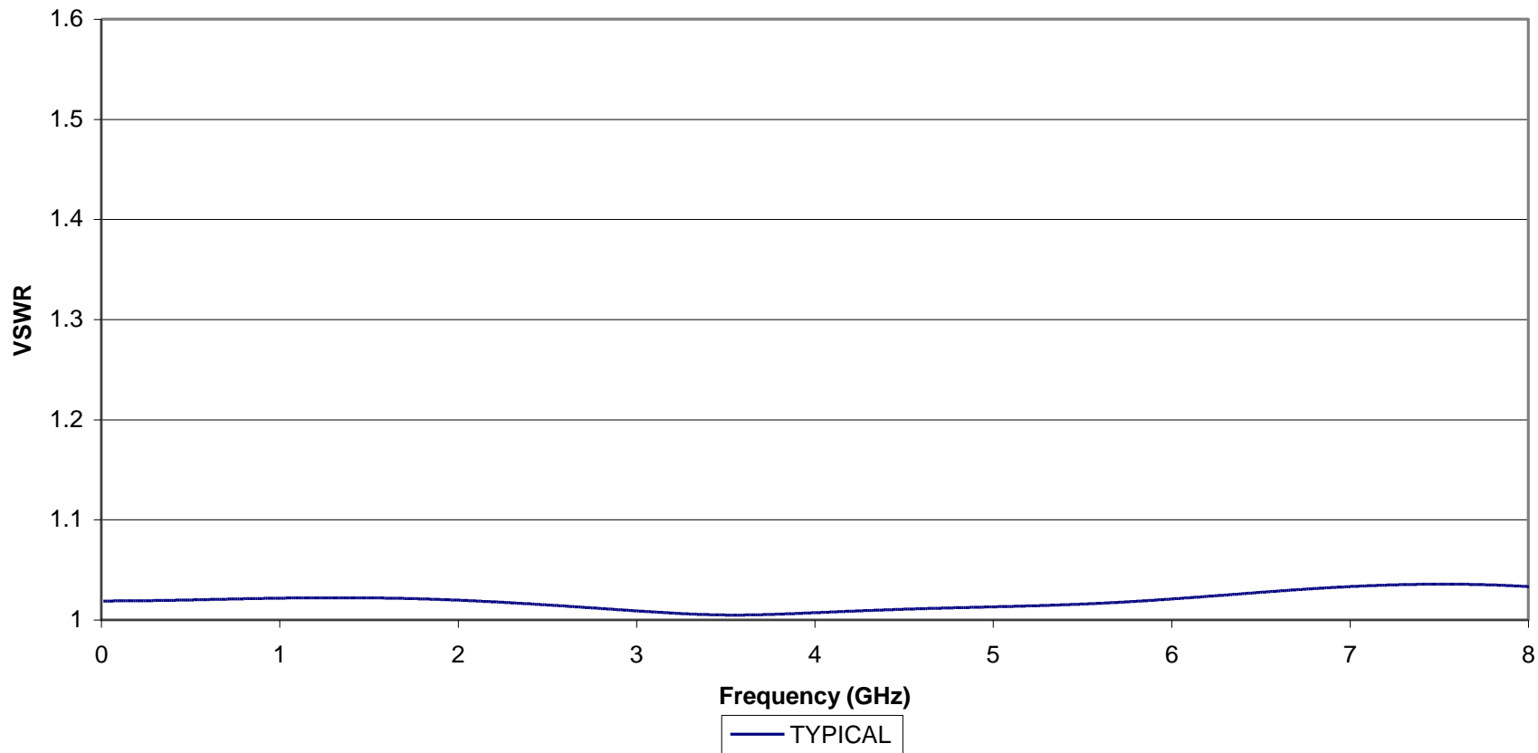
TYPICAL VSWR OF KOAXXA SMA-JB-1D (1-2081204-1) RG-178 Cable
