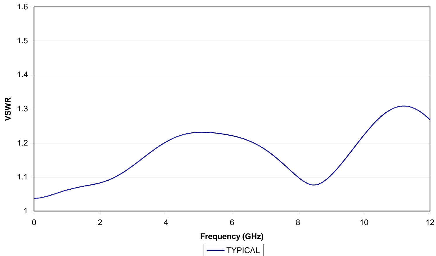
TYPICAL VSWR OF KOAXXA SMA-PR-1G (2081203-7) RG-58 Cable
