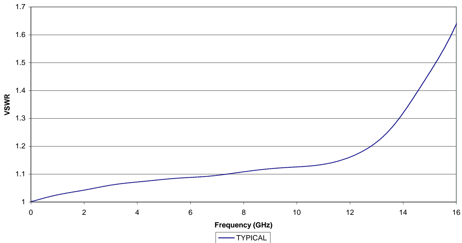
TYPICAL VSWR OF KOAXXA SMA-PR-1A (2081203-1) RG-402 Cable
